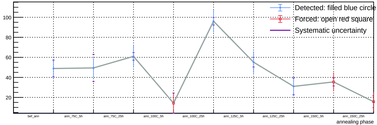
Sensor A1, T = 20\text{ C} , v_{\text{over}} = 7\text{ V} - Spot 40: luminosity vs phase
