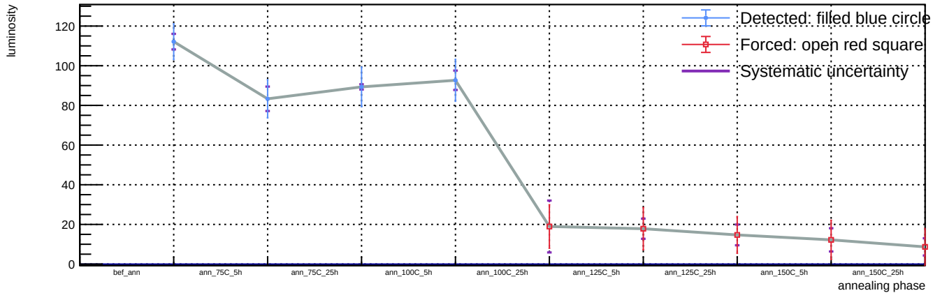
Sensor A1, T = 20\text{ C} , v_{\text{over}} = 7\text{ V} - Spot 41: luminosity vs phase
