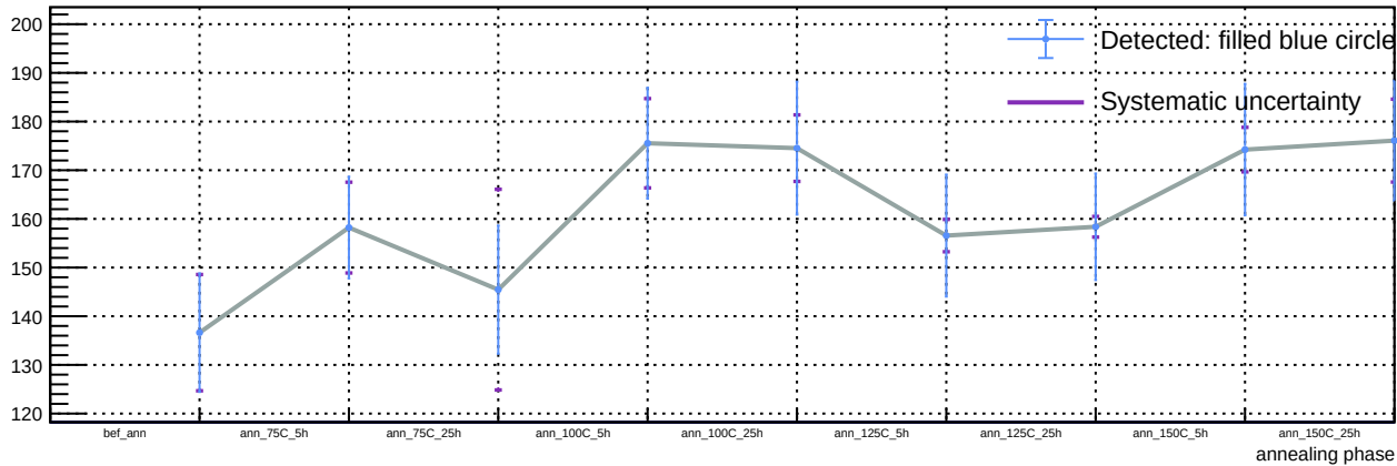
Sensor A1, T = 20\text{ C} , v_{\text{over}} = 7\text{ V} - Spot 42: luminosity vs phase
