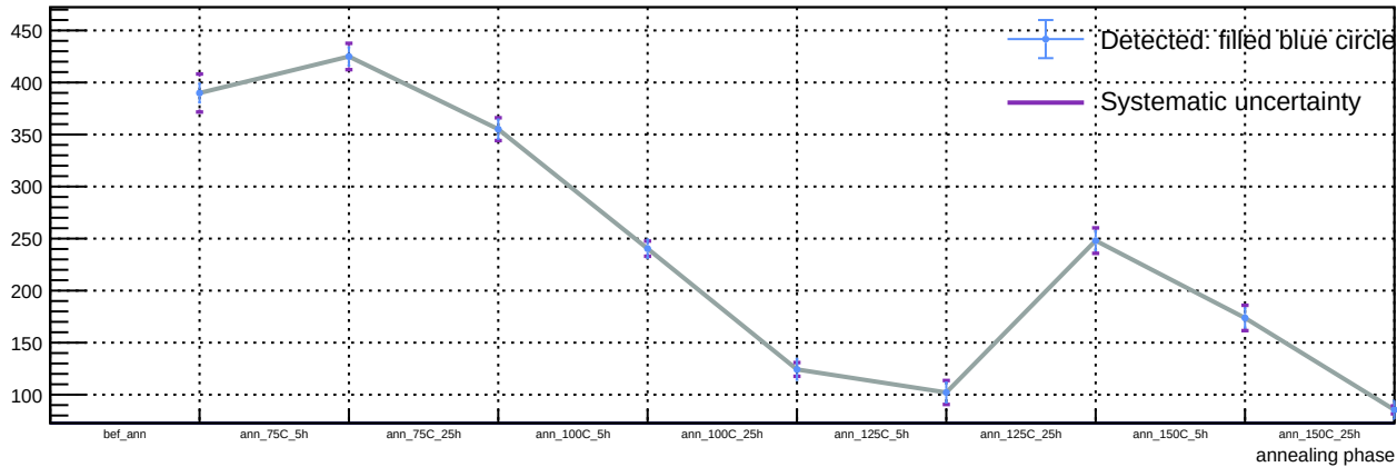
Sensor A1, T = 20\text{ C} , v_{\text{over}} = 7\text{ V} - Spot 45: luminosity vs phase
