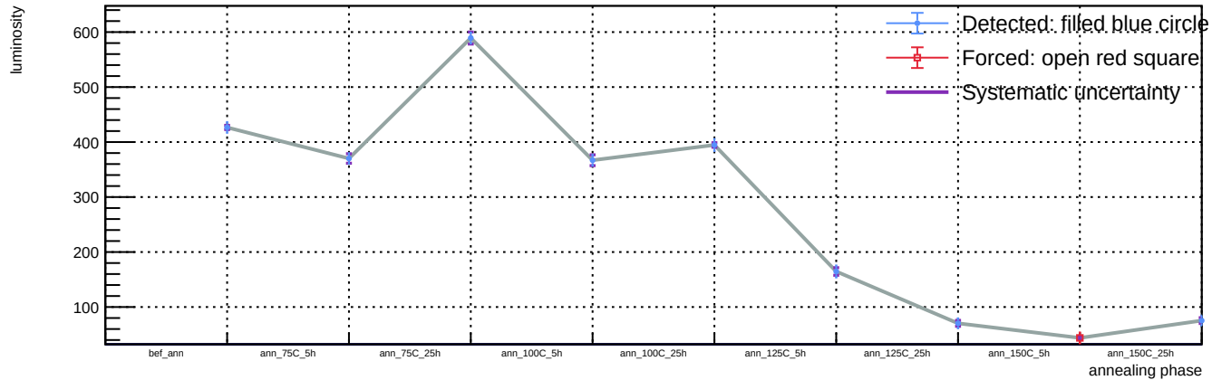
Sensor A1, T = 20\text{ C} , v_{\text{over}} = 7\text{ V} - Spot 46: luminosity vs phase
