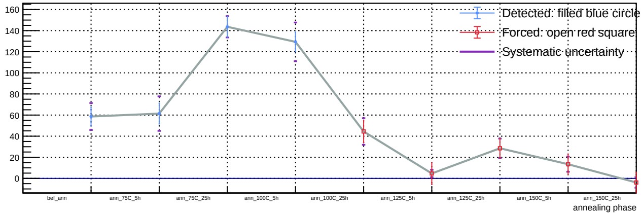
Sensor A1, T = 20\text{ C} , v_{\text{over}} = 7\text{ V} - Spot 47: luminosity vs phase
