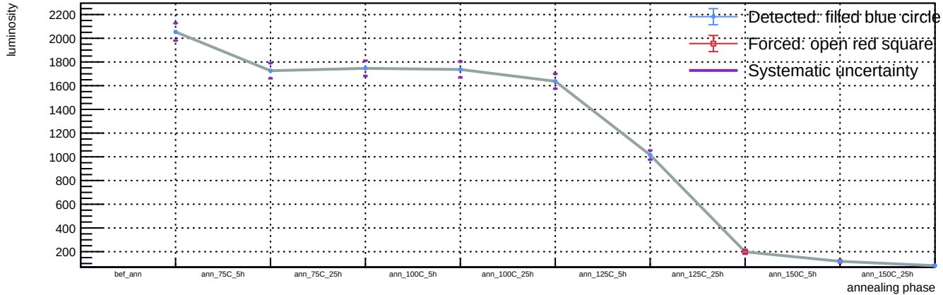
Sensor A1, T = 20\text{ C} , v_{\text{over}} = 7\text{ V} - Spot 48: luminosity vs phase
