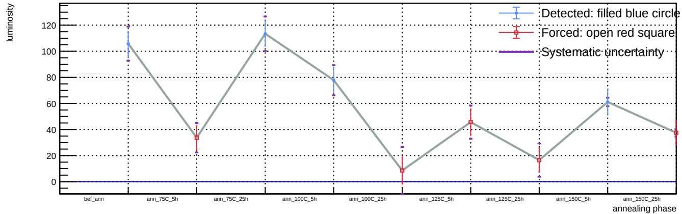
Sensor A1, T = 20\text{ C} , v_{\text{over}} = 7\text{ V} - Spot 5: luminosity vs phase
