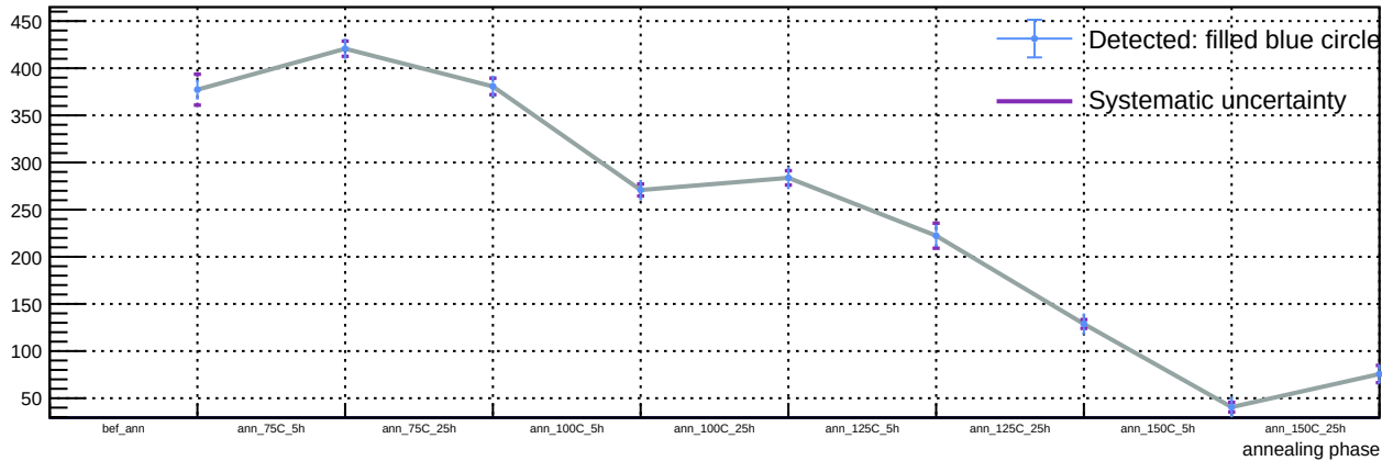
Sensor A1, T = 20\text{ C} , v_{\text{over}} = 7\text{ V} - Spot 56: luminosity vs phase
