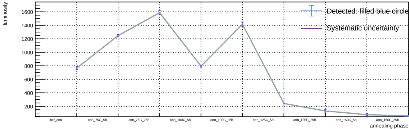
Sensor A1, T = 20\text{ C} , v_{\text{over}} = 7\text{ V} - Spot 59: luminosity vs phase
