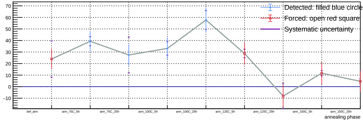
Sensor A1, T = 20\text{ C} , v_{\text{over}} = 7\text{ V} - Spot 60: luminosity vs phase
