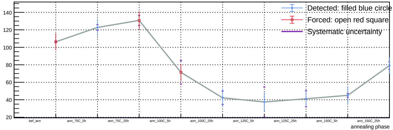
Sensor A1, T = 20\text{ C} , v_{\text{over}} = 7\text{ V} - Spot 61: luminosity vs phase
