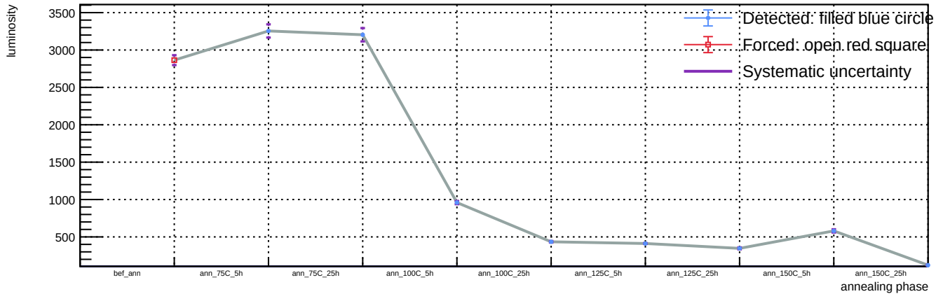
Sensor A1, T = 20\text{ C} , v_{\text{over}} = 7\text{ V} - Spot 62: luminosity vs phase
