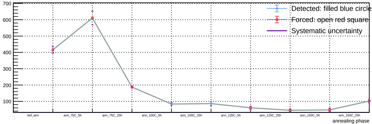
Sensor A1, T = 20\text{ C} , v_{\text{over}} = 7\text{ V} - Spot 69: luminosity vs phase
