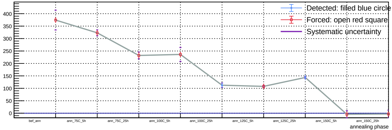
Sensor A1, T = 20\text{ C} , v_{\text{over}} = 7\text{ V} - Spot 75: luminosity vs phase
