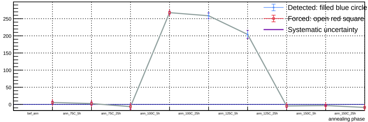
Sensor A1, T = 20\text{ C} , v_{\text{over}} = 7\text{ V} - Spot 78: luminosity vs phase
