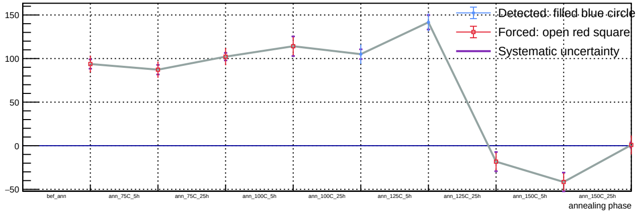
Sensor A1, T = 20\text{ C} , v_{\text{over}} = 7\text{ V} - Spot 79: luminosity vs phase
