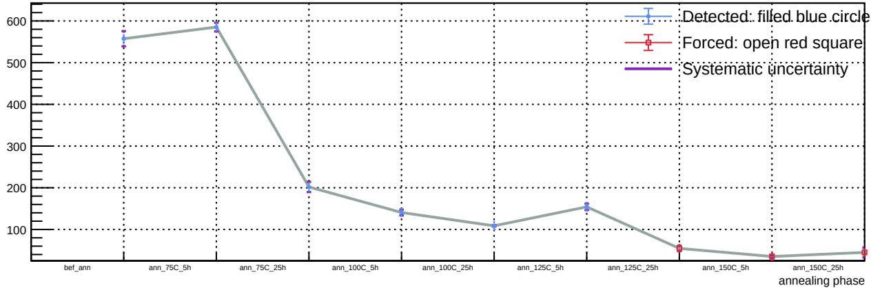
Sensor A1, T = 20\text{ C} , v_{\text{over}} = 7\text{ V} - Spot 8: luminosity vs phase
