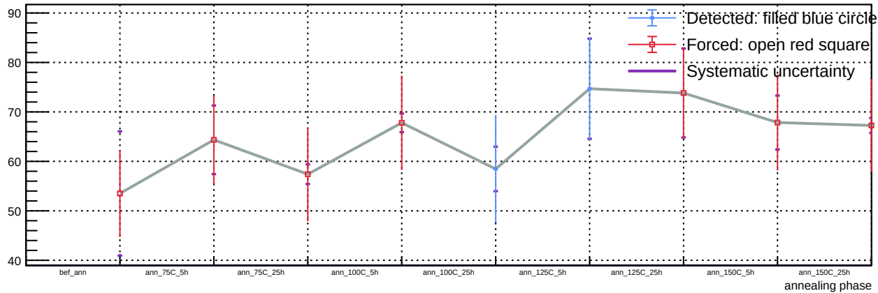
Sensor A1, T = 20\text{ C} , v_{\text{over}} = 7\text{ V} - Spot 80: luminosity vs phase
