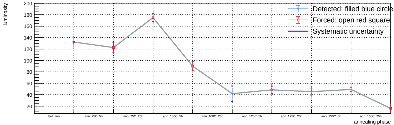
Sensor A1, T = 20\text{ C} , v_{\text{over}} = 7\text{ V} - Spot 81: luminosity vs phase
