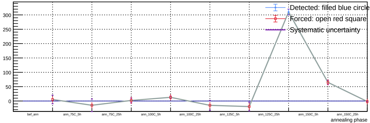
Sensor A1, T = 20\text{ C} , v_{\text{over}} = 7\text{ V} - Spot 83: luminosity vs phase
