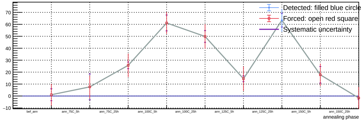
Sensor A1, T = 20\text{ C} , v_{\text{over}} = 7\text{ V} - Spot 84: luminosity vs phase
