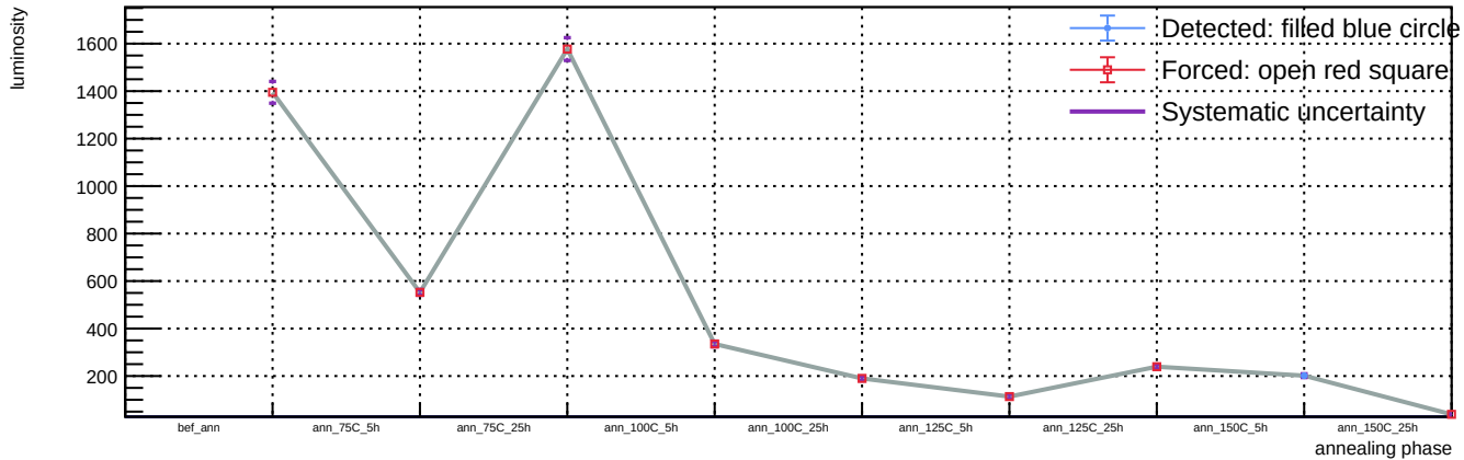
Sensor A1, T = 20\text{ C} , v_{\text{over}} = 7\text{ V} - Spot 87: luminosity vs phase
