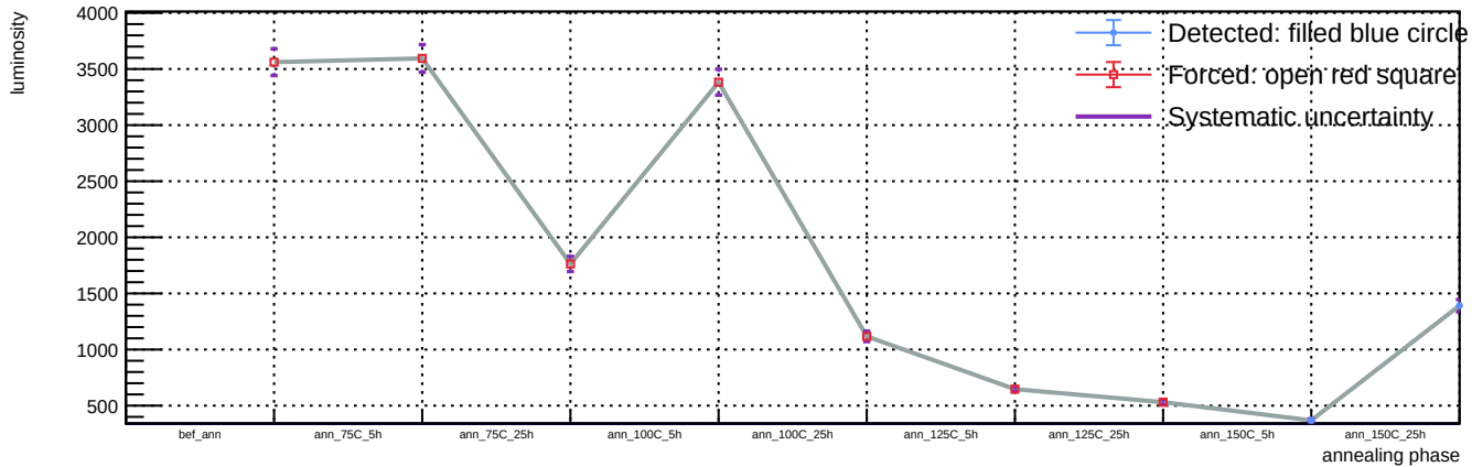
Sensor A1, T = 20\text{ C} , v_{\text{over}} = 7\text{ V} - Spot 88: luminosity vs phase
