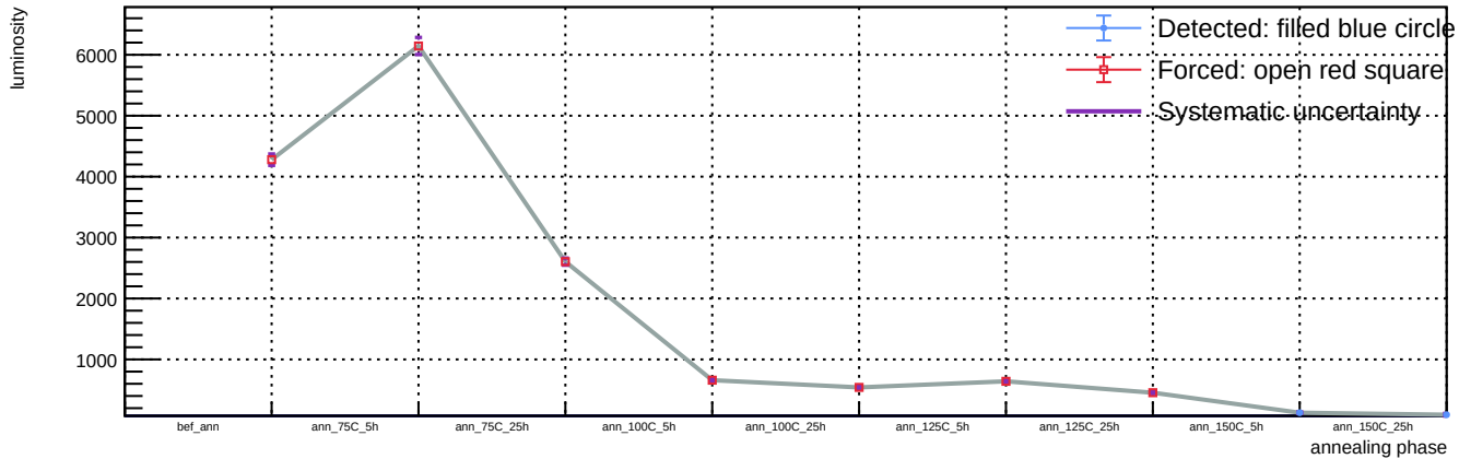
Sensor A1, T = 20\text{ C} , v_{\text{over}} = 7\text{ V} - Spot 92: luminosity vs phase
