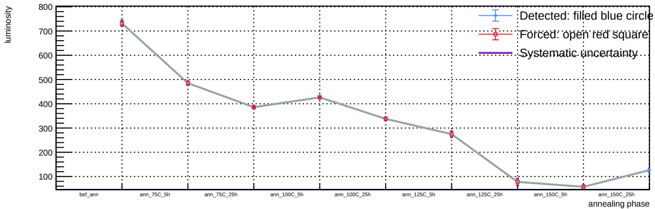
Sensor A1, T = 20\text{ C} , v_{\text{over}} = 7\text{ V} - Spot 93: luminosity vs phase
