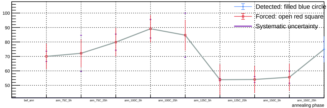
Sensor A1, T = 20\text{ C} , v_{\text{over}} = 7\text{ V} - Spot 96: luminosity vs phase
