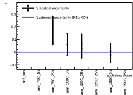
Sensor A1, v = 5 V - Spot 68
