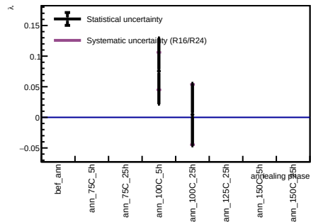
Sensor A1, v = 5 V - Spot 66
