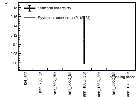
Sensor A1, v = 5 V - Spot 69
