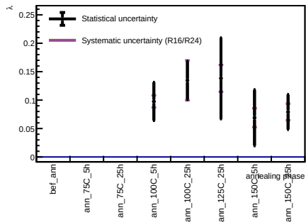
Sensor A1, v = 5 V - Spot 70
