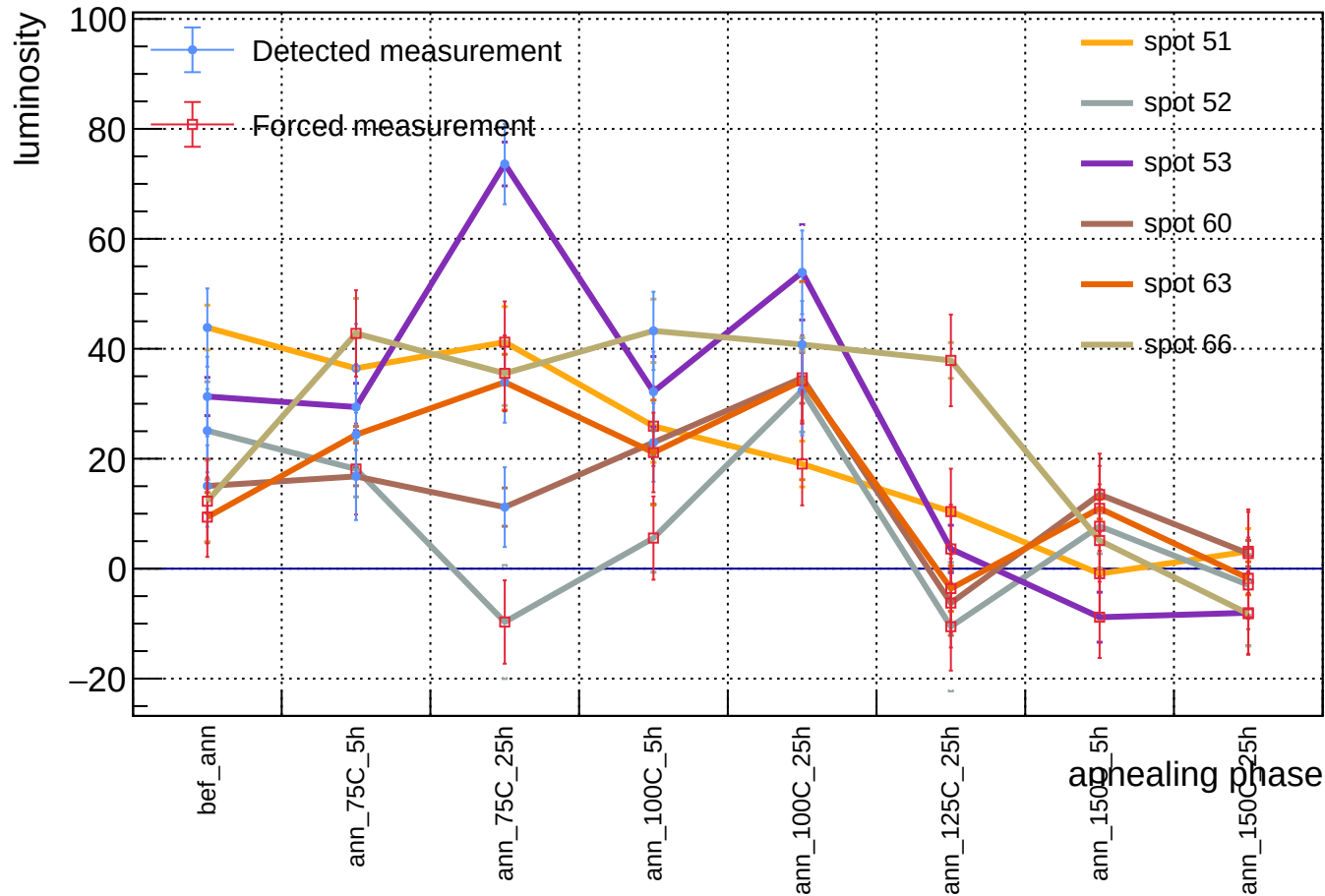
Sensor A1, v = 5 V, T = 23 °C - luminosity vs phase - order 10^1
