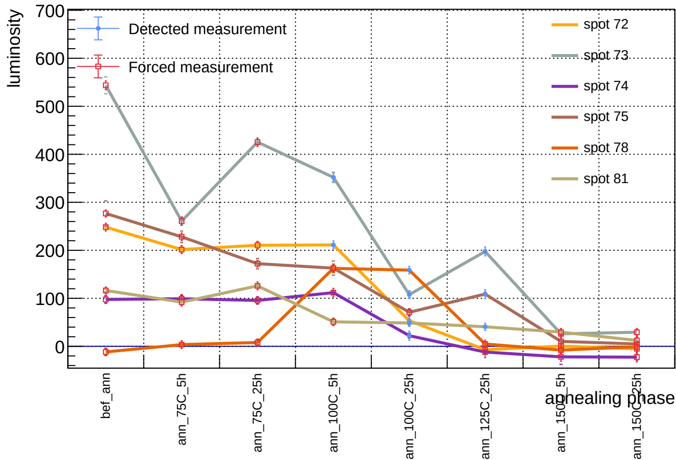
Sensor A1, v = 5 V, T = 23 °C - luminosity vs phase - order 10^2
