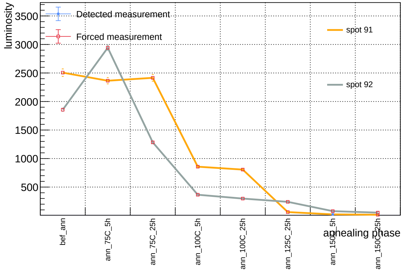
Sensor A1, v = 5 V, T = 23 °C - luminosity vs phase - order 10^3
