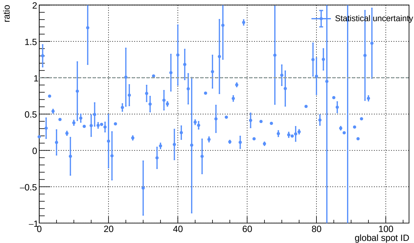
Sensor A1, v = 5 V - L(\text{ann\_100C\_25h}) / L(\text{before\_annealing})
