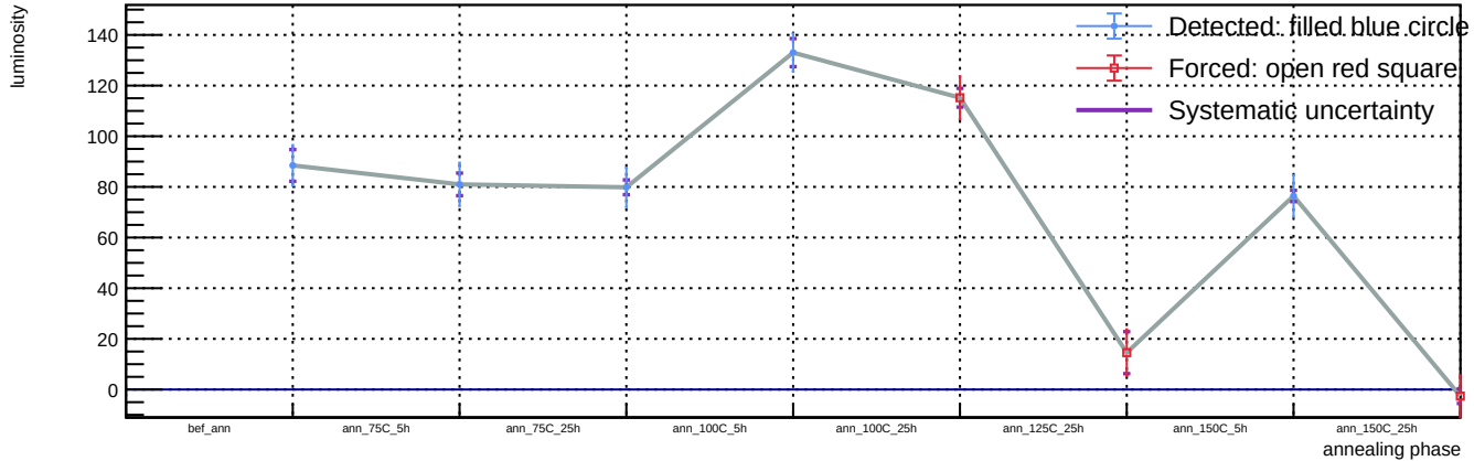
Sensor A1, v = 5 V, T = 23 °C - Spot 1: luminosity vs phase
