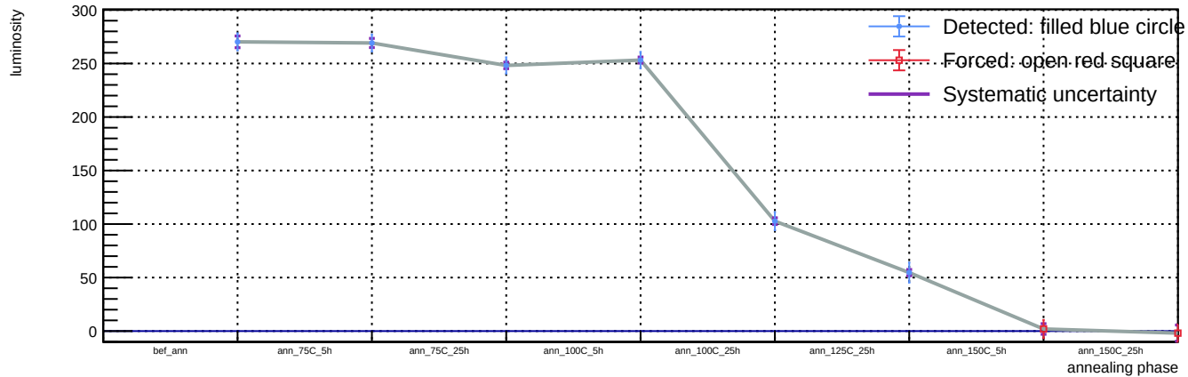
Sensor A1, v = 5 V, T = 23 °C - Spot 10: luminosity vs phase
