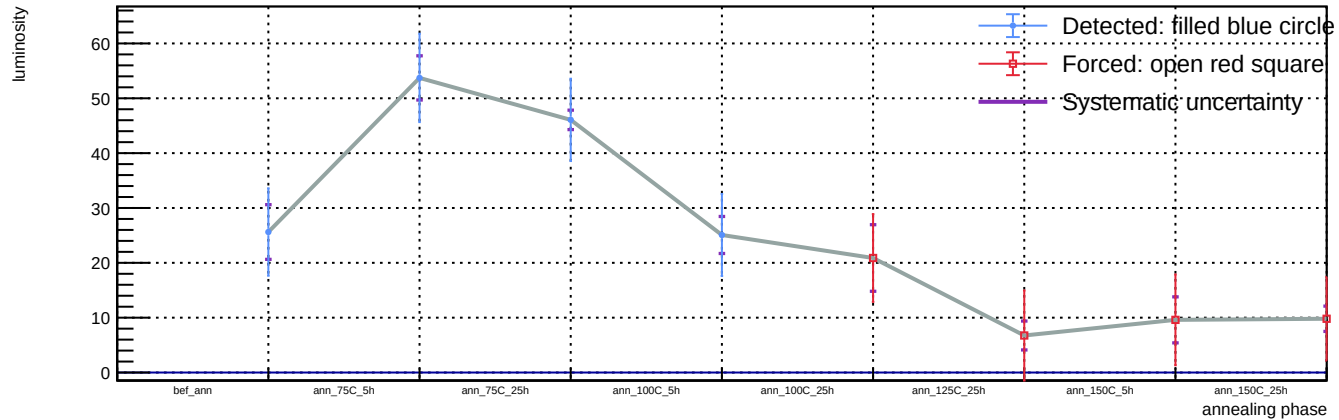
Sensor A1, v = 5 V, T = 23 °C - Spot 11: luminosity vs phase
