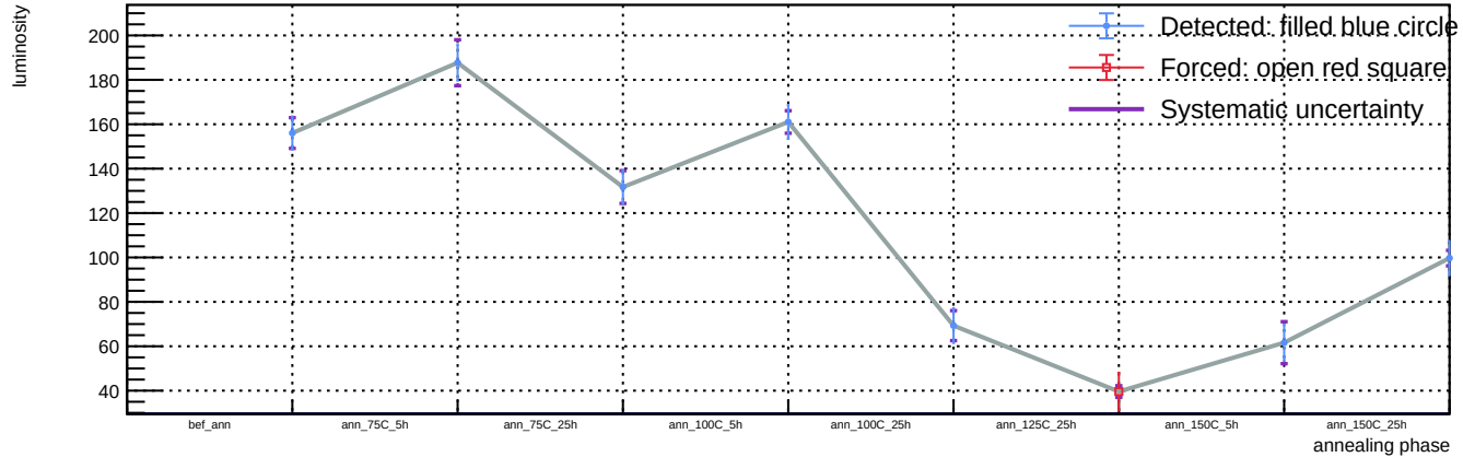
Sensor A1, v = 5 V, T = 23 °C - Spot 12: luminosity vs phase
