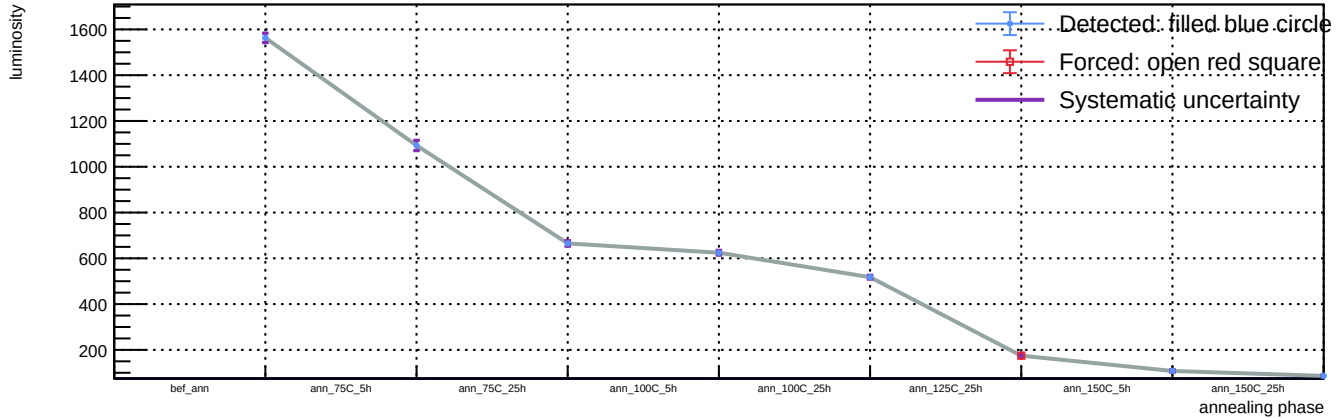
Sensor A1, v = 5 V, T = 23 °C - Spot 13: luminosity vs phase
