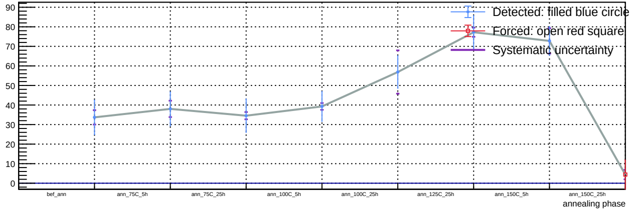
Sensor A1, v = 5 V, T = 23 °C - Spot 14: luminosity vs phase
