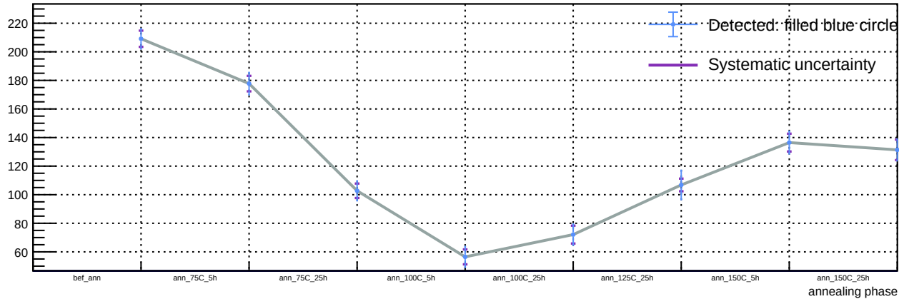
Sensor A1, v = 5 V, T = 23 °C - Spot 17: luminosity vs phase
