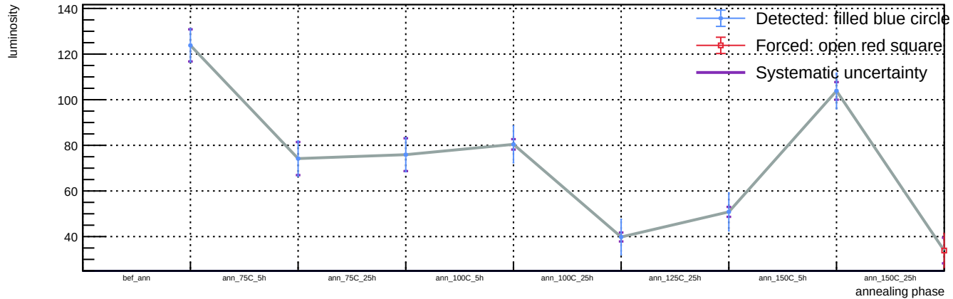
Sensor A1, v = 5 V, T = 23 °C - Spot 19: luminosity vs phase
