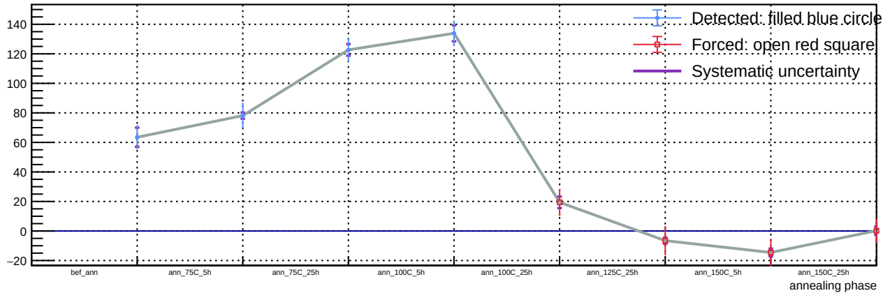
Sensor A1, v = 5 V, T = 23 °C - Spot 2: luminosity vs phase
