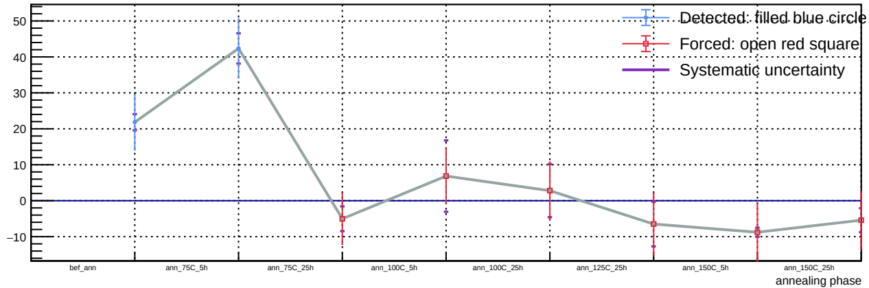
Sensor A1, v = 5 V, T = 23 °C - Spot 20: luminosity vs phase
