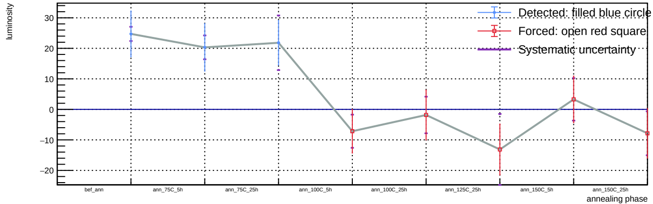
Sensor A1, v = 5 V, T = 23 °C - Spot 21: luminosity vs phase
