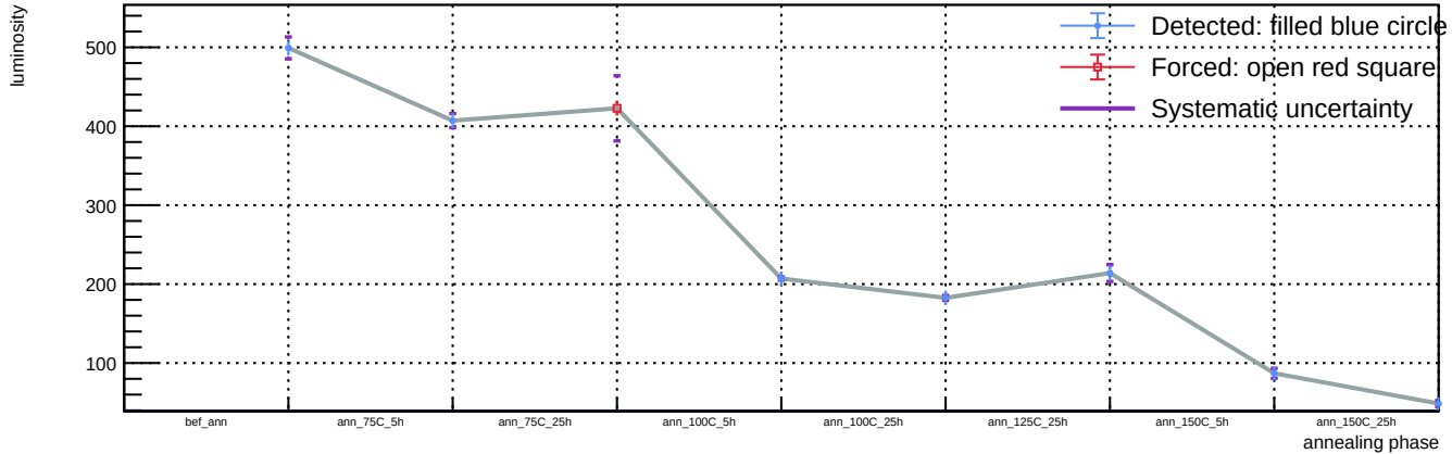
Sensor A1, v = 5 V, T = 23 °C - Spot 22: luminosity vs phase
