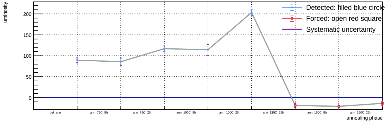
Sensor A1, v = 5 V, T = 23 °C - Spot 23: luminosity vs phase
