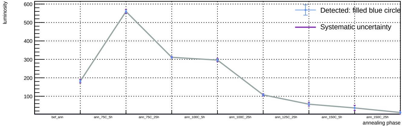
Sensor A1, v = 5 V, T = 23 °C - Spot 24: luminosity vs phase
