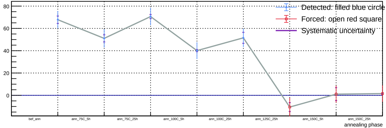
Sensor A1, v = 5 V, T = 23 °C - Spot 26: luminosity vs phase
