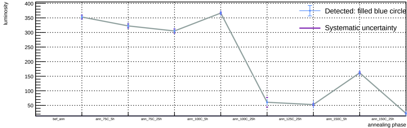
Sensor A1, v = 5 V, T = 23 °C - Spot 27: luminosity vs phase
