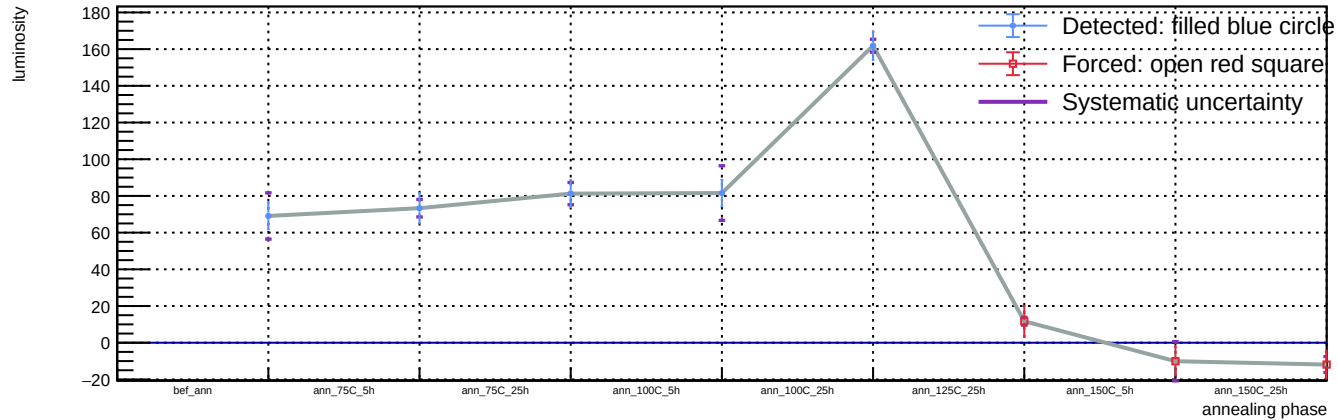
Sensor A1, v = 5 V, T = 23 °C - Spot 28: luminosity vs phase
