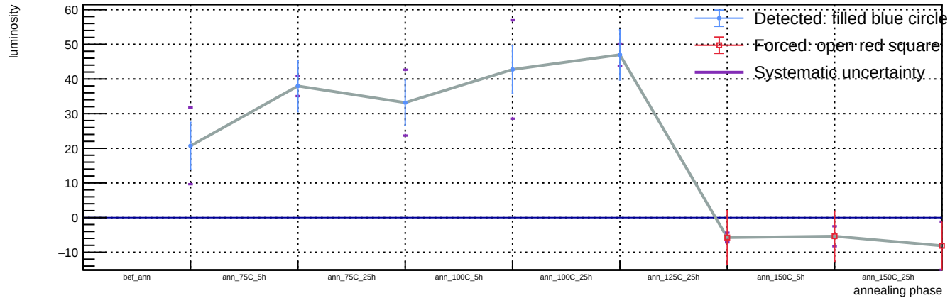
Sensor A1, v = 5 V, T = 23 °C - Spot 29: luminosity vs phase
